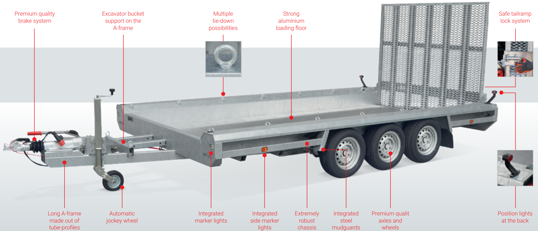
Extremely strong platform support because of the many bearers
